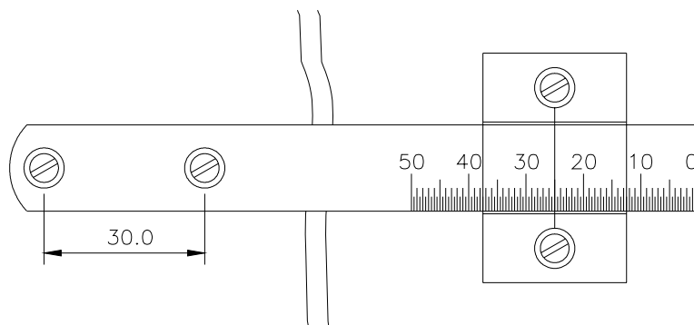
Model EDJ-40C crackmeter
